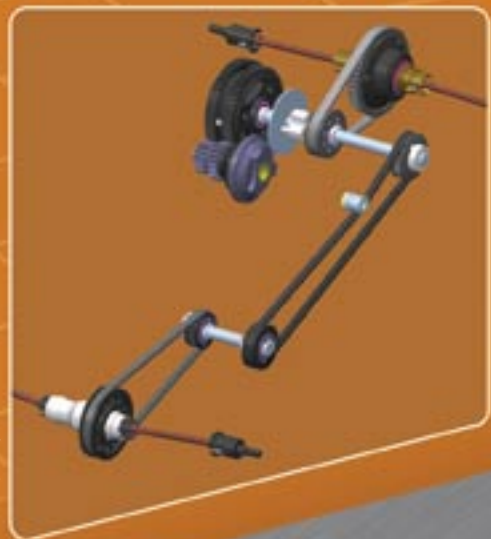
Ball differential using an innovative clamping collar to allow quick and easy adjustment. (Front ball diff optional)
